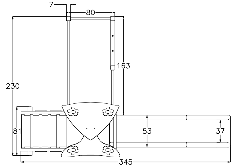
PIANTA (PLAN)
