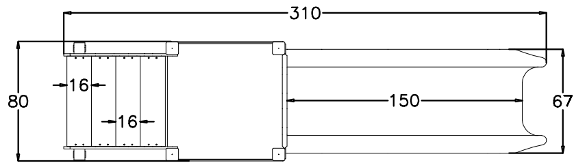
PIANTA (PLAN)
