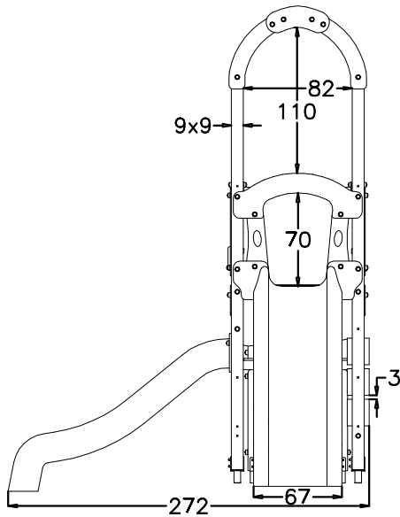
VISTA FRONTALE (FRONTAL VIEW)
