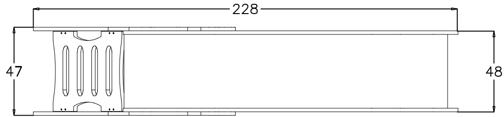
PIANTA (PLAN)
