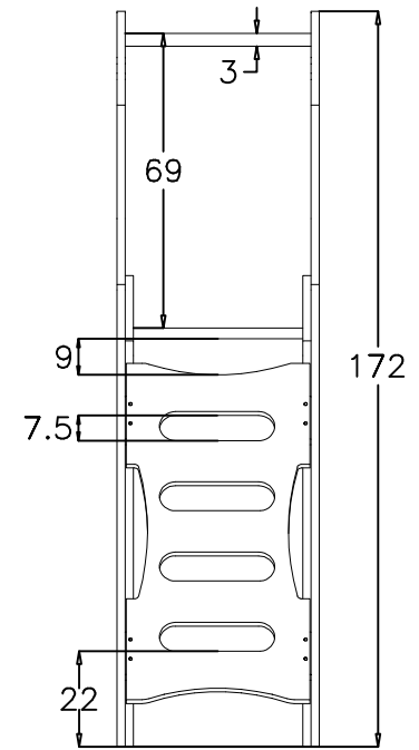
VISTA FRONTALE (FRONTAL VIEW)
