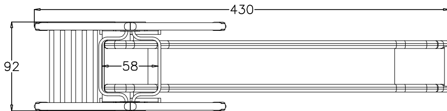
PIANTA (PLAN)
