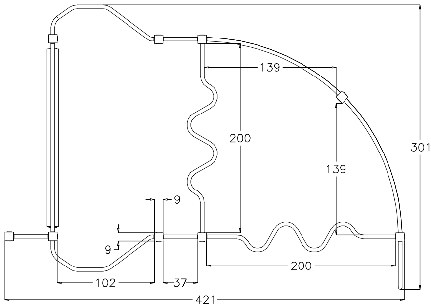
PIANTA (PLAN)
