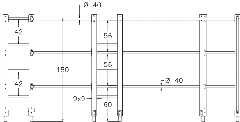
FRONTALE (FRONTAL)
