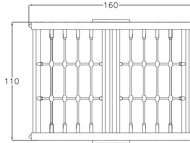
PIANTA (PLAN)
