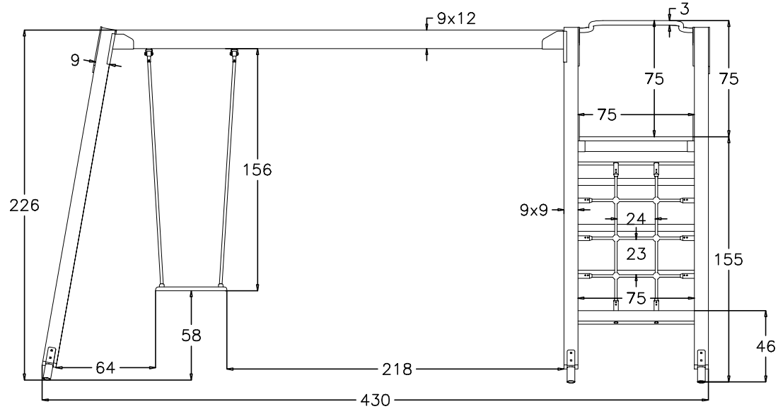
VISTA LATERALE (LATERAL VIEW)
