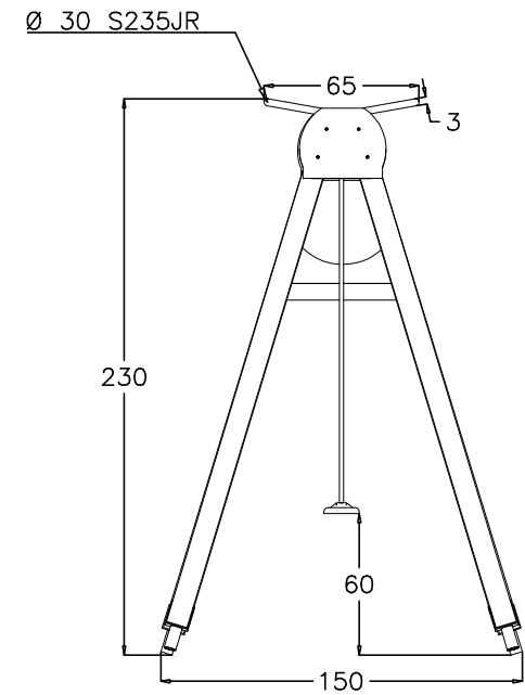
VISTA FRONTALE (FRONTAL VIEW)
